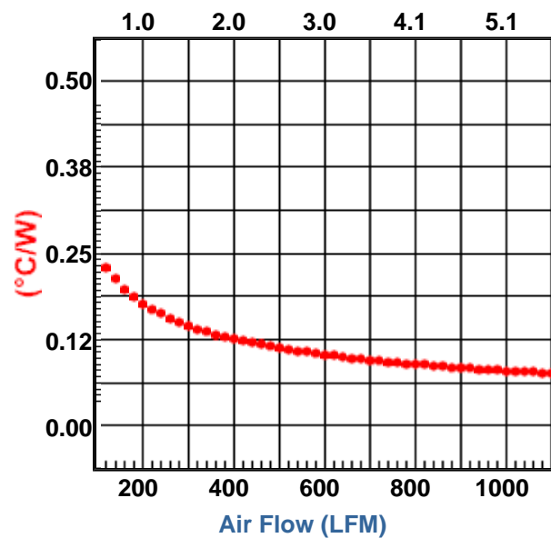
Heat Sink Thermal Resistance (100W Dissipated)
